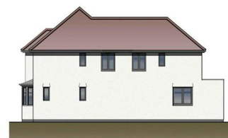
WEST ELEVATION - 1:100
